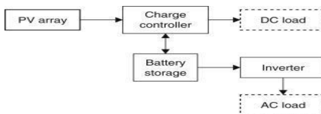
Fig 5.10 Solar PV System Block Diagram
